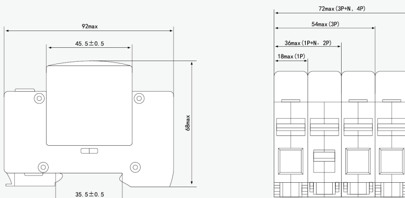
Figure 3 Outline and Installation Dimensions of Type C Surge Protection Device
