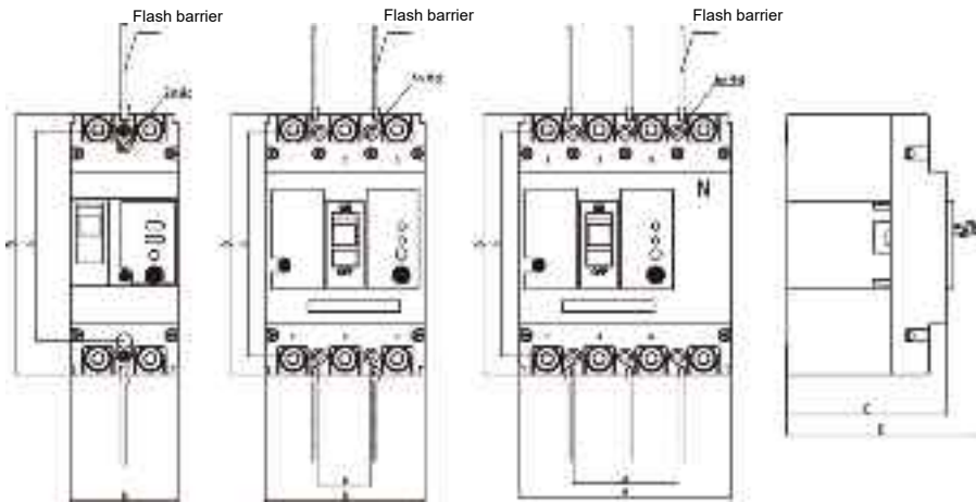
Figure 3 Outline and installation dimensions
