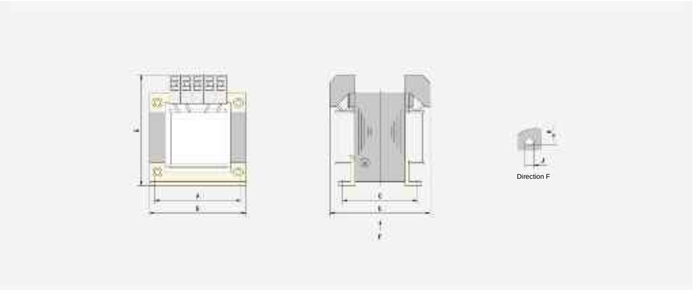
4. Outline and installation dimension diagram of JBK4
