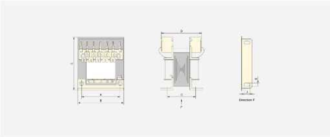
3. Outline and installation dimension diagram of JBK3
